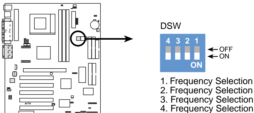
A7V DIP Switches
