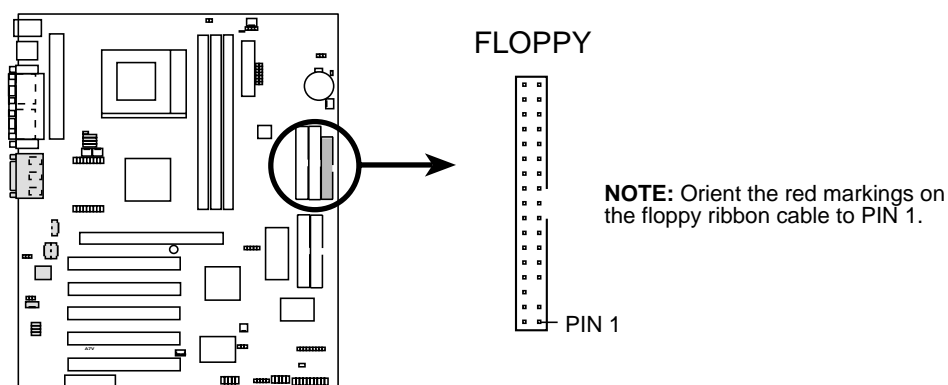
A7V Floppy Disk Drive Connector
