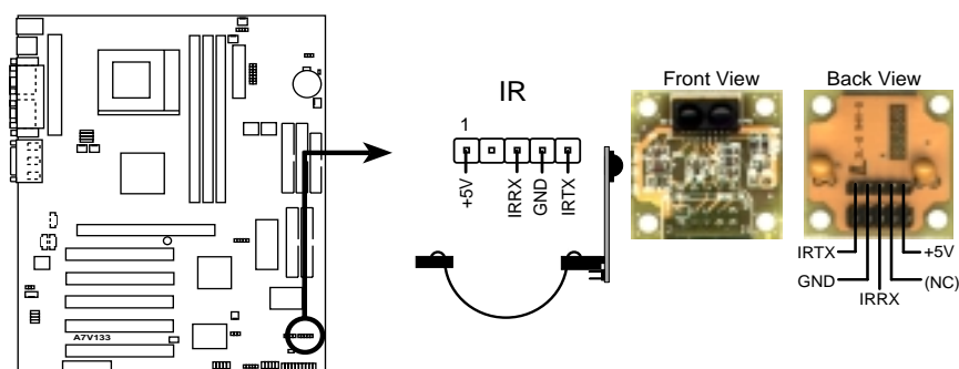
A7V133 Infrared Module Connector
