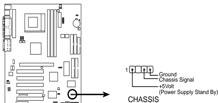
A7V133 Chassis Open Alarm Lead
