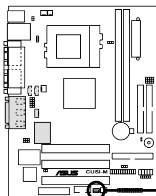
CUSI-M Wake-On-LAN Connector
