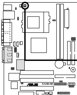
CUSI-M Wake On Ring Connector
