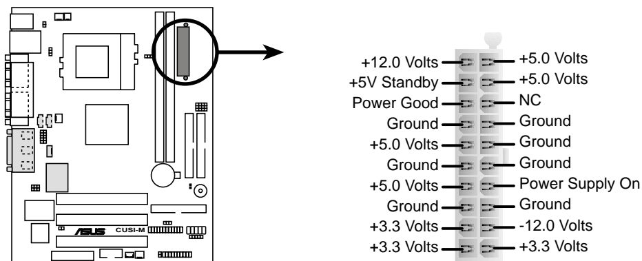
CUSI-M ATX Power Connector
