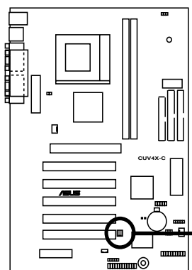
CUV4X-C Wake-On-Ring Connector
