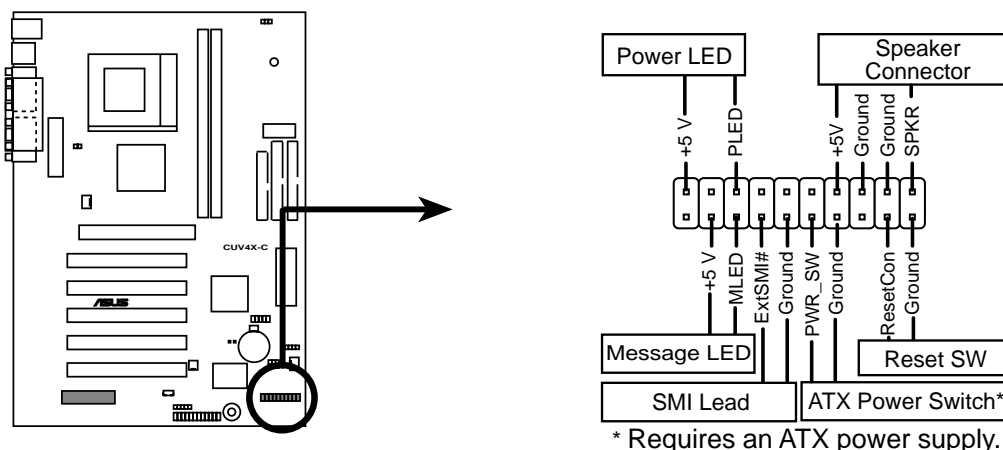
CUV4X-C System Panel Connectors
