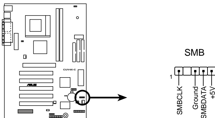
CUV4X-C SMBus Connector
