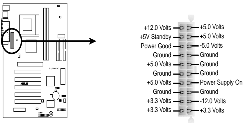
CUV4X-C ATX Power Connector
