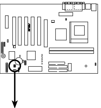
CUV4X-C JumperFree™ Mode Setting
