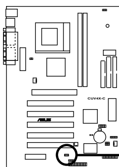
CUV4X-C Wake-On-LAN Connector
