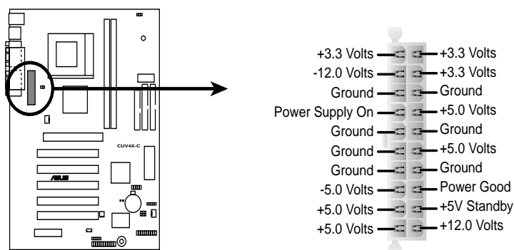
CUV4X-C ATX Power Connector
