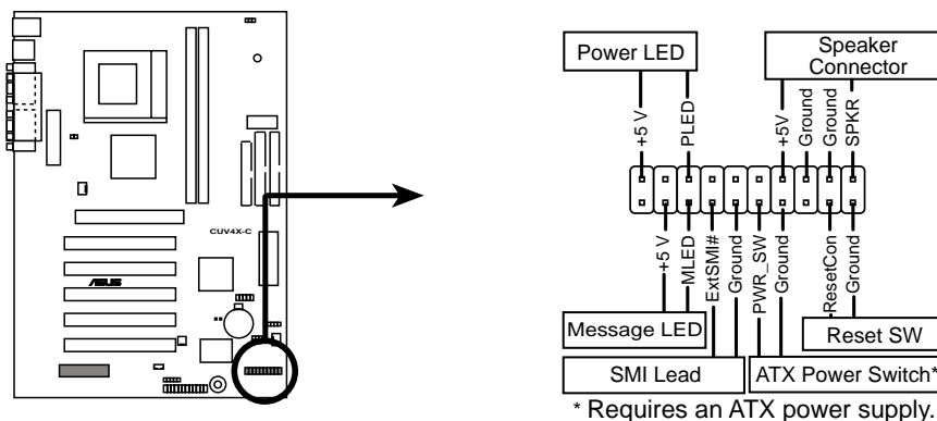
CUV4X-C System Panel Connectors
