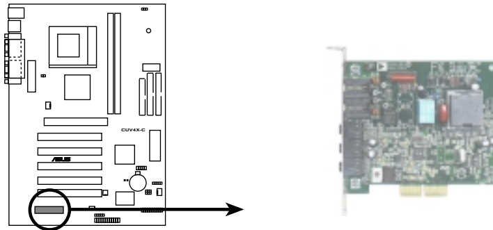
CUV4X-C Audio Modem Riser (AMR) Connector
