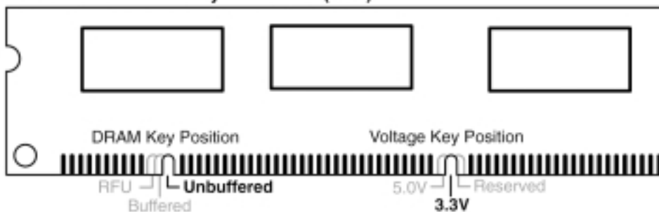
168-Pin DIMM Notch Key Definitions (3.3V)
