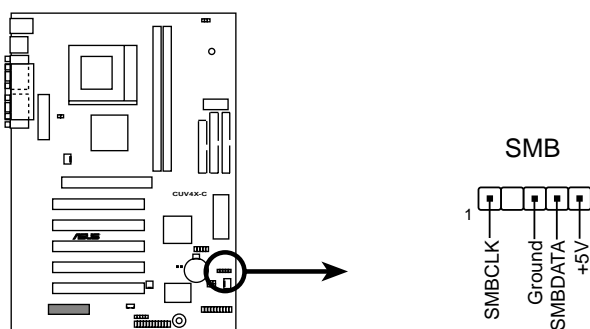
CUV4X-C SMBus Connector
