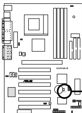
CUV4X-E Clear RTC RAM
