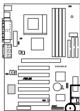
CUV4X-E IDE Activity LED
