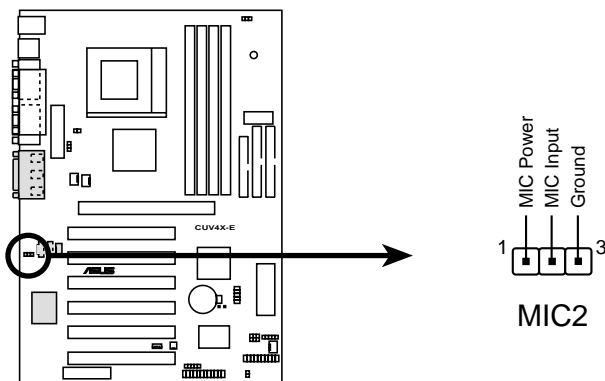
CUV4X-E Internal Microphone Connector
