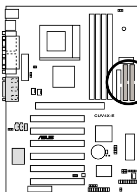
CUV4X-E IDE Connectors
