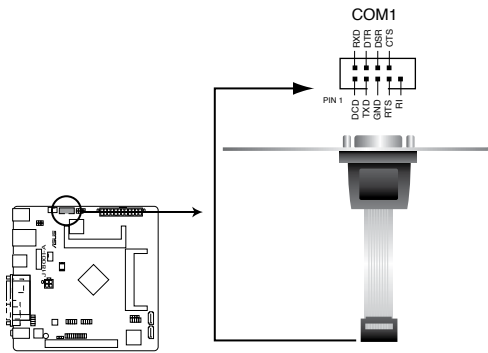
J1800I-A Serial port connector
