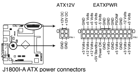
J1800I-A ATX power connectors
