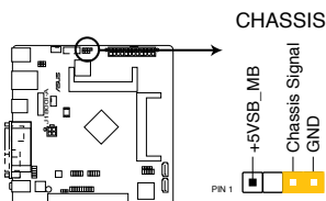
J1800I-A Chassis intrusion connector
