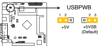
J1800I-A Keyboard and USB device wake up
