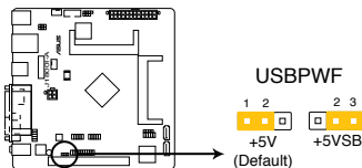
J1800I-A USB device wake up
