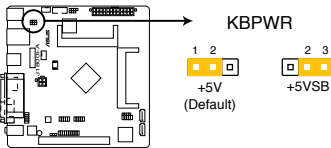
J1800I-A Keyboard Power Setting
