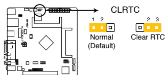
J1800I-A Clear RTC RAM
