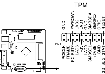
J1800I-A TPM Connector
