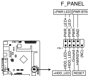
J1800I-A System panel connector
