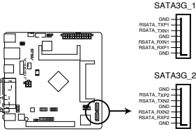
J1800I-A SATA 3.0Gb/s connectors
