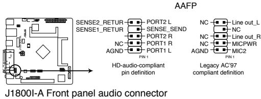
J1800I-A Front panel audio connector
