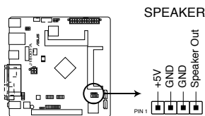
J1800I-A Speaker Out Connector
