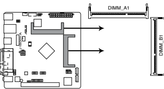
J1800I-A 204-pin DDR3 DIMM sockets
