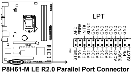
P8H61-M LE R2.0 Parallel Port Connector
