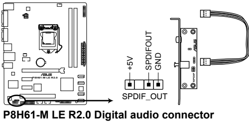
P8H61-M LE R2.0 Digital audio connector
