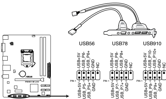
P8H61-M LX3 USB2.0 connectors
