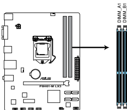
P8H61-M LX3 240-pin DDR3 DIMM sockets
