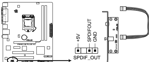
P8H61-M PLUS V3 Digital audio connector
