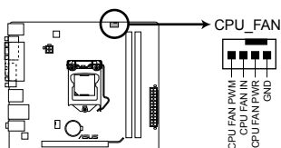
P8H61-M PLUS V3 CPU fan connector
