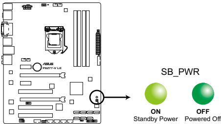
P8Z77-V LE Onboard LED
