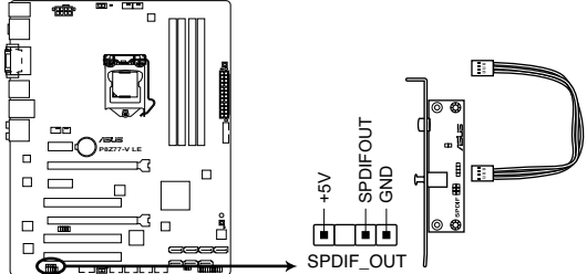
P8Z77-V LE Digital audio connector
