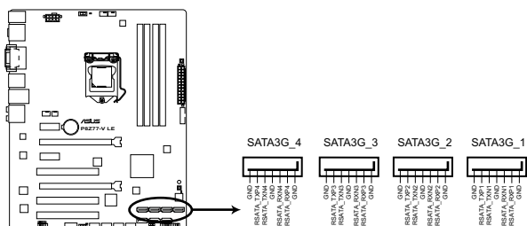
P8277-V LE SATA 3.0Gb/s connectors
