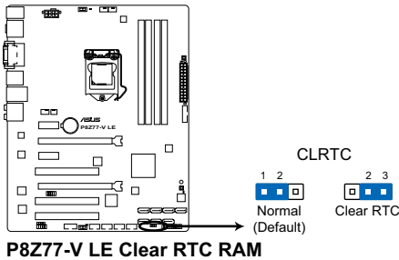
P8Z77-V LE Clear RTC RAM
