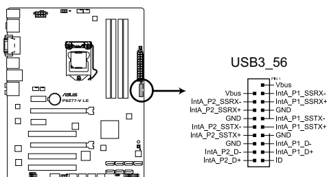
P8277-V LE USB3.0 Front panel connector
