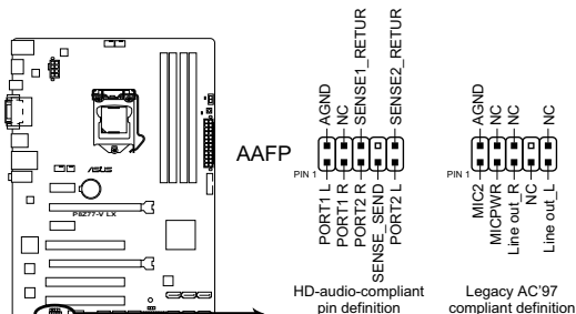
P8Z77-V LX Front panel audio connector
