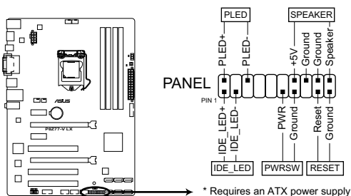
P8Z77-V LX System panel connector
