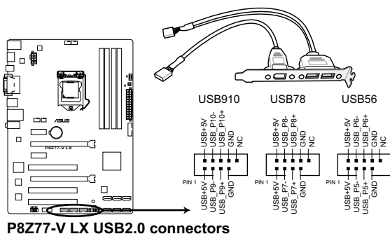
P8Z77-V LX USB2.0 connectors
