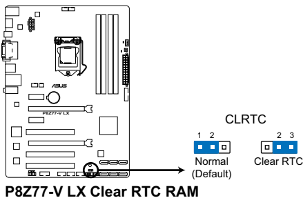
P8Z77-V LX Clear RTC RAM
