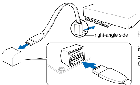
P8Z77 WS Intel® SATA 6.0 Gb/s connectors
