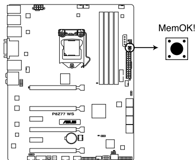
P8Z77 WS MemOK! switch
