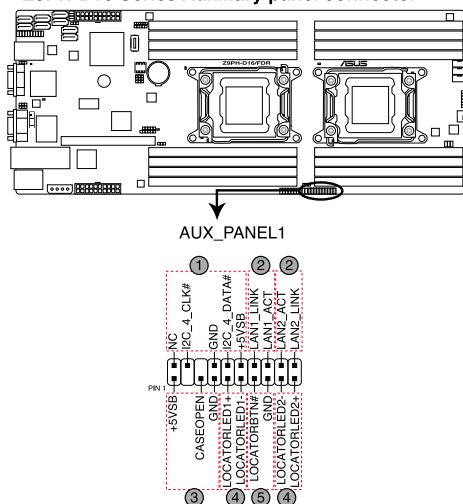
Z9PH-D16 Series Auxiliary panel connector
