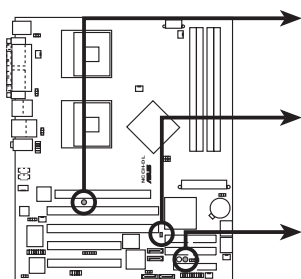
NCCH-DL Warning LEDs
