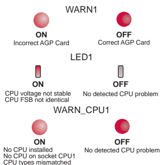
NCCH-DL Warning LEDs
