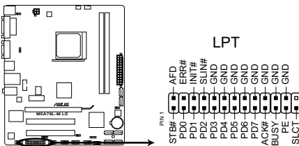
M5A78L-M LE LPT connector
