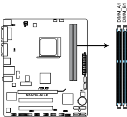
M5A78L-M LE 240-pin DDR3 DIMM sockets
