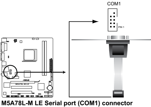
M5A78L-M LE Serial port (COM1) connector
