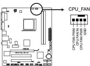
M5A78L-M LE CPU fan connector
