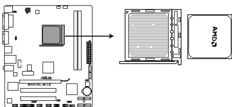
M5A78L-M LE CPU socket AM3+
