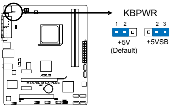
M5A78L-M LX PLUS Keyboard power setting
