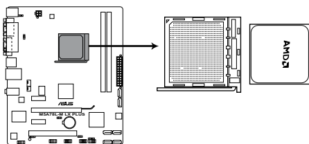
M5A78L-M LX PLUS CPU AM3+
