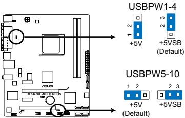
M5A78L-M LX PLUS USB device wake-up
