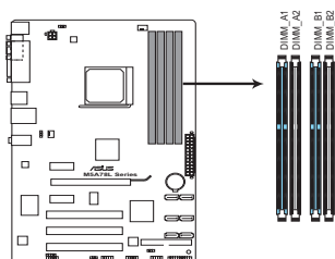
Sockets DIMM DDR3 de la M5A78L Series
