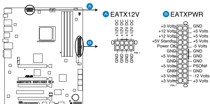
SABERTOOTH 990FX/GEN3 R2.0 ATX power connectors
