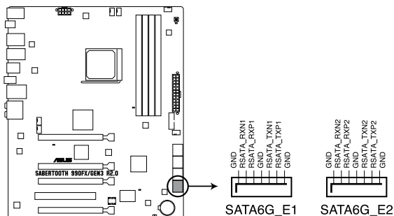
SABERTOOTH 990FX/GEN3 R2.0 ASMedia® SATA 6.0 Gb/s connectors
