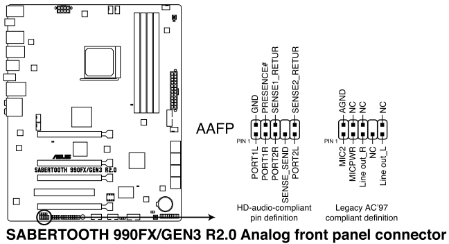
SABERTOOTH 990FX/GEN3 R2.0 Analog front panel connector
