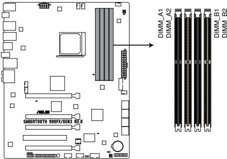
SABERTOOTH 990FX/GEN3 R2.0 240-pin DDR3 DIMM slots
