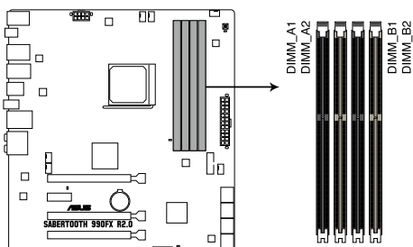
SABERTOOTH 990FX R2.0 240-pin DDR3 DIMM socket
