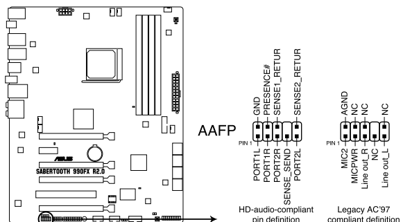
SABERTOOTH 990FX R2.0 Analog front panel connector
