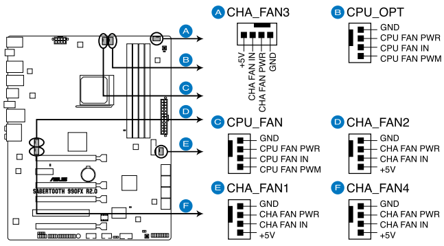
SABERTOOTH 990FX R2.0 Fan connectors
