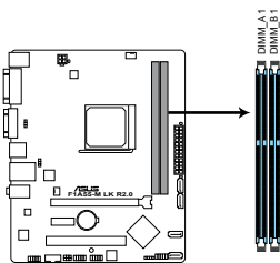
F1A55-M LK R2.0 240-pin DDR3 DIMM sockets
