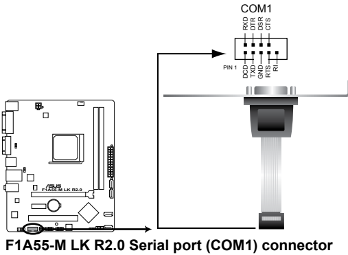
F1A55-M LK R2.0 Serial port (COM1) connector
