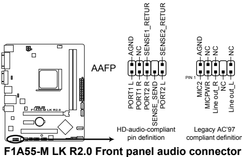
F1A55-M LK R2.0 Front panel audio connector
