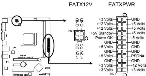
F1A55-M LX3 R2.0 ATX power connectors
