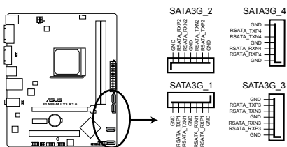
F1A55-M LX3 R2.0 SATA 3.0Gb/s connectors
