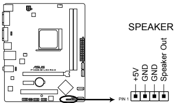
F1A55-M LX3 R2.0 Speaker Out Connector
