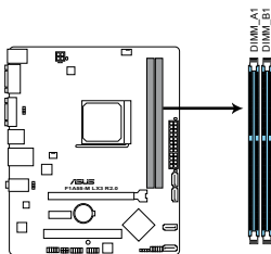
F1A55-M LX3 R2.0 240-pin DDR3 DIMM sockets
