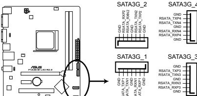
F1A55-M LX3 R2.0 SATA 3.0Gb/s connectors
