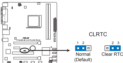
F1A55-M LX PLUS R2.0 Clear RTC RAM
