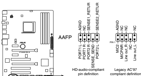
F1A55 R2.0 Front panel audio connector
