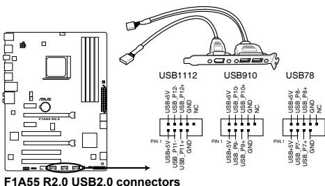
F1A55 R2.0 USB2.0 connectors
