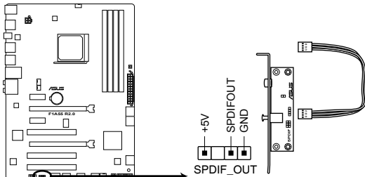
F1A55 R2.0 Digital audio connector
