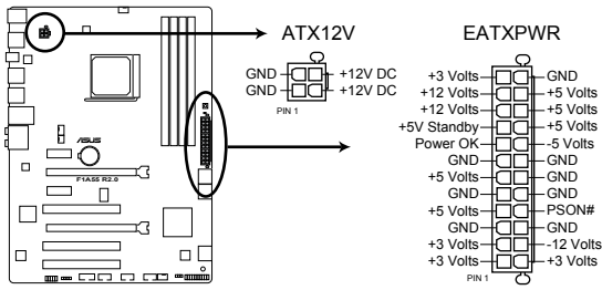
F1A55 R2.0 ATX power connectors
