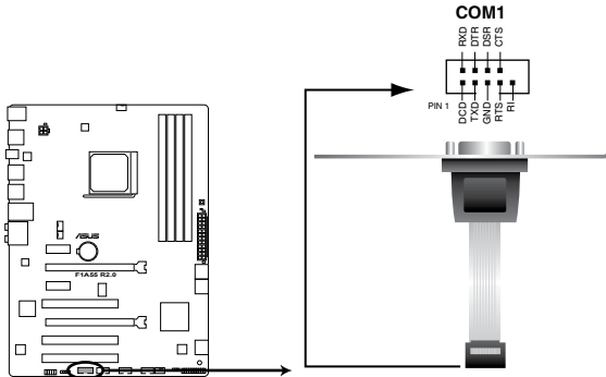
F1A55 R2.0 Serial port (COM1) connector
