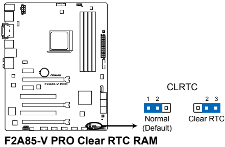
F2A85-V PRO Clear RTC RAM
