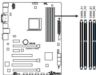
F2A85-V PRO 240-pin DDR3 DIMM sockets
