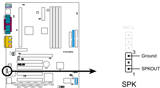
P3C2000 Internal Speaker Connector
