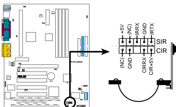
P3C2000 Infrared Module Connector
