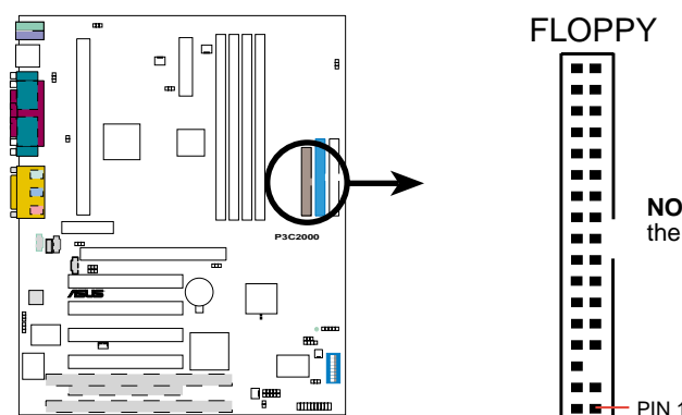
P3C2000 Floppy Disk Drive Connector
