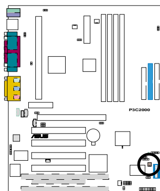
P3C2000 Wake-On-Ring Connector
