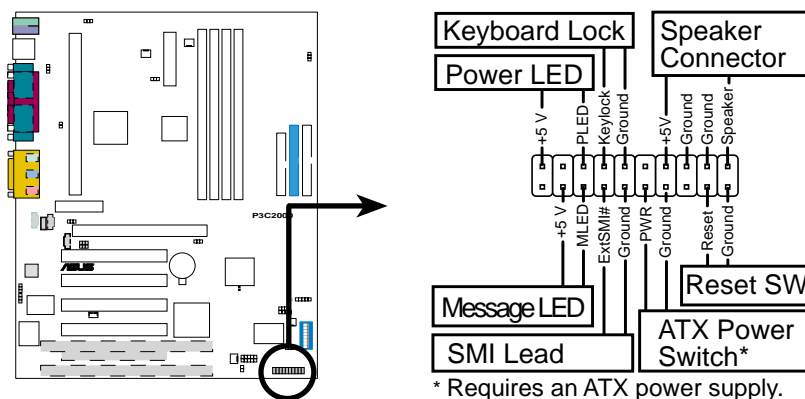
P3C2000 System Panel Connectors
