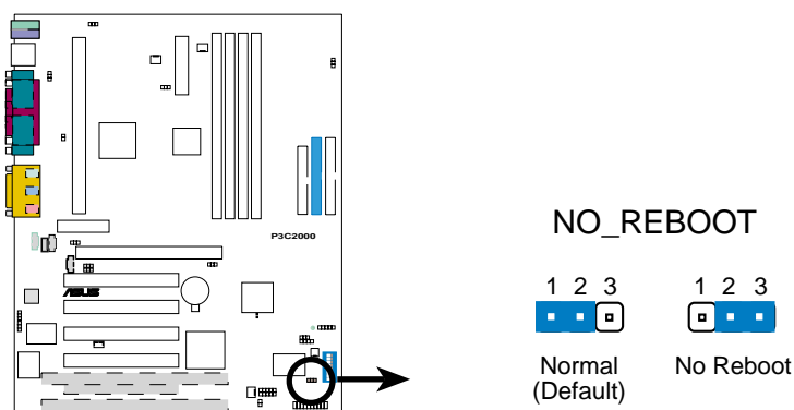
P3C2000 Reboot Setting
