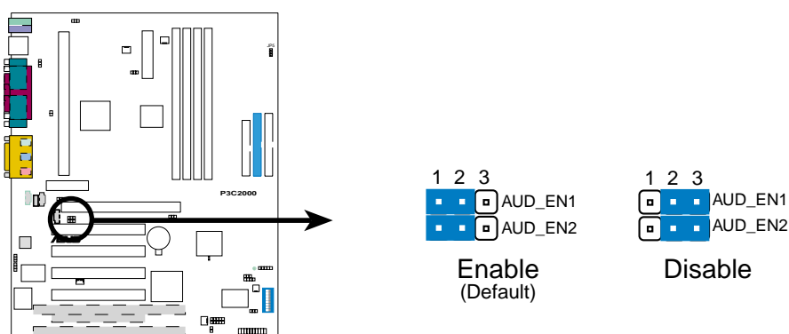
P3C2000 Audio Codec Setting
