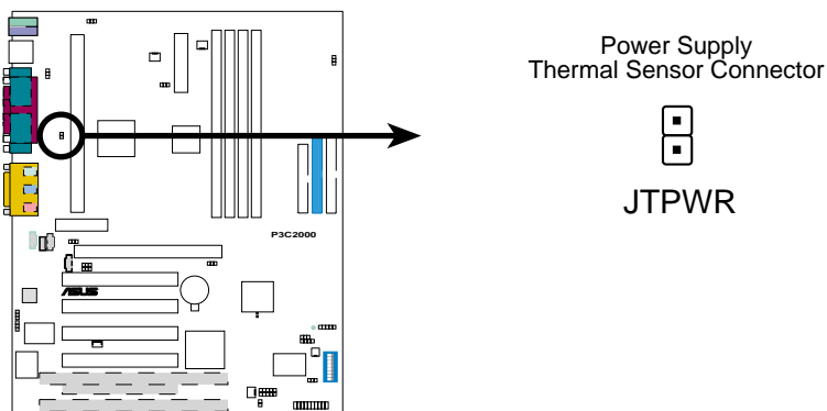
P3C2000 Thermal Sensor Connector
