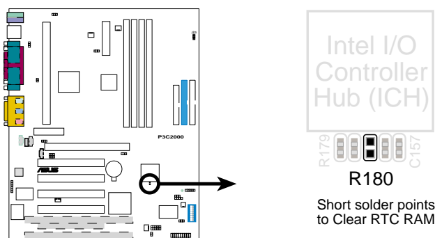
P3C2000 Clear RTC RAM
