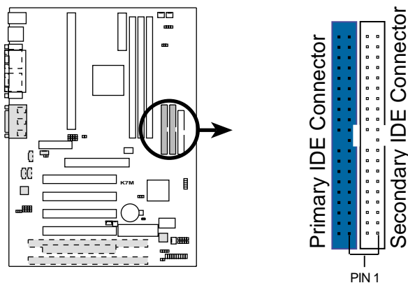
K7M IDE Connectors
