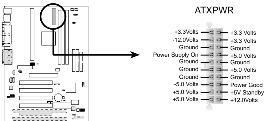
K7M ATX Power Connector
