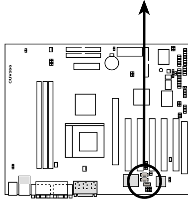
CUV266 Internal Audio Connectors
