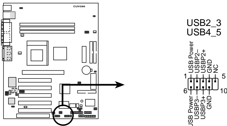
CUV266 Front Panel USB Headers
