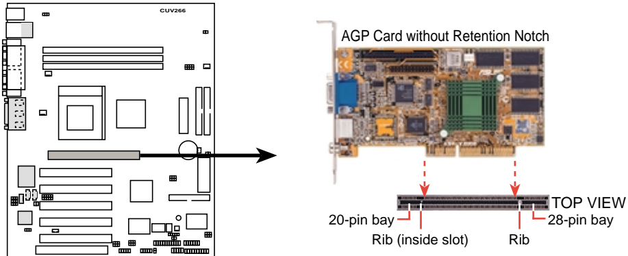
CUV266 Accelerated Graphics Port (AGP PRO)
