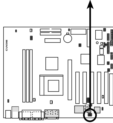
CUV266 Internal Microphone Connector
