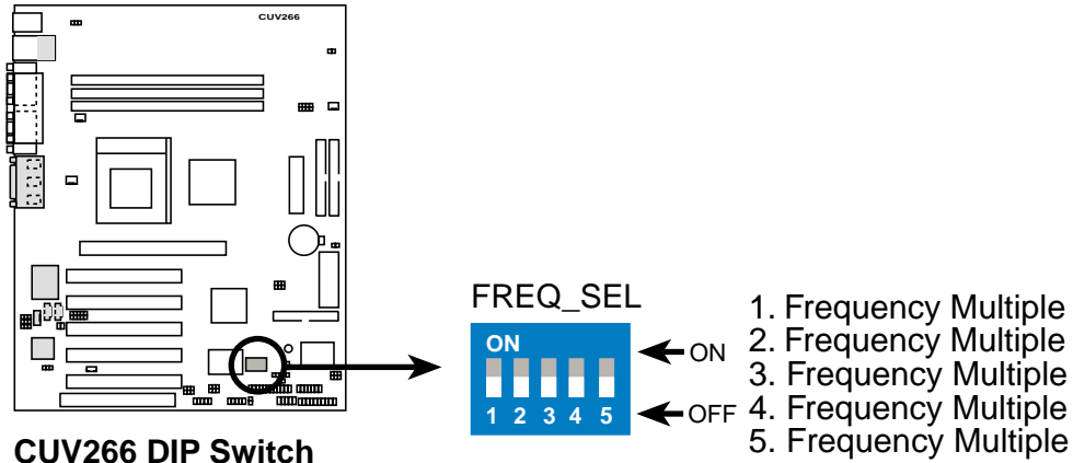
CUV266 DIP Switch
