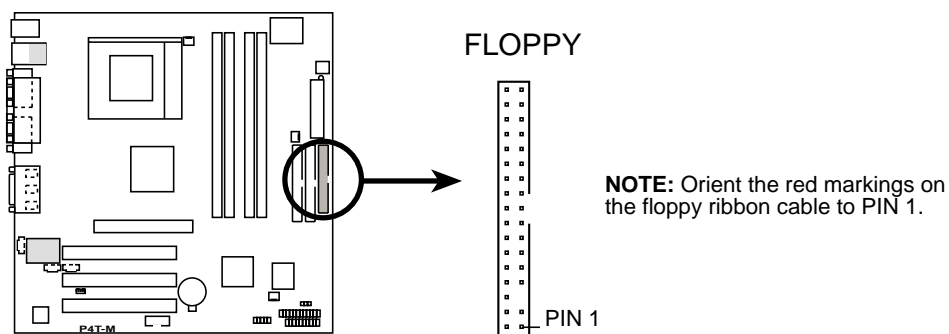
P4T-M Floppy Disk Drive Connector
