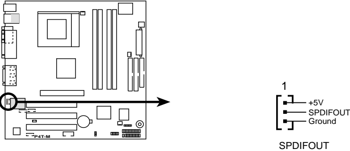
P4T-M Digital Audio Interface
