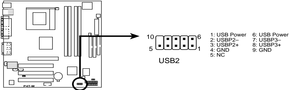
P4T-M USB Headers
