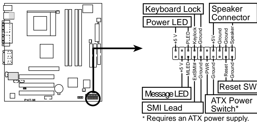
P4T-M System Panel Connectors
