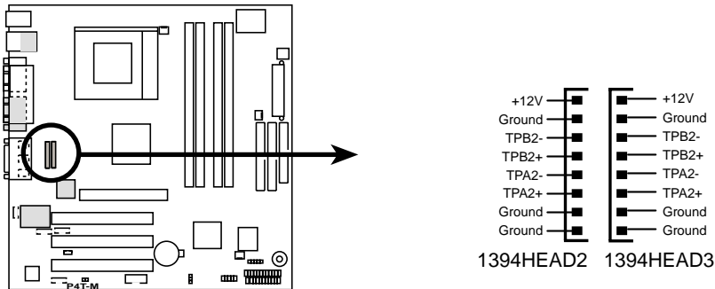
P4T-M IEEE-1394 Headers
