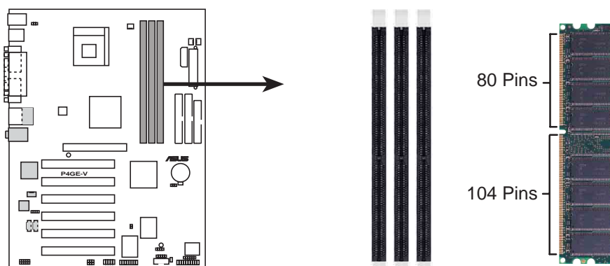
P4GE-V 184-Pin DDR DIMM Sockets
