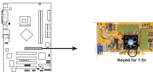
P4P800S-X Accelerated Graphics Port (AGP)
