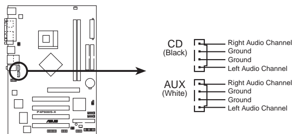
P4P800S-X Internal Audio Connectors
