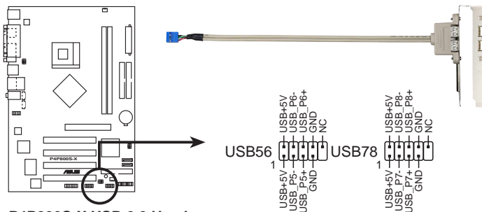
P4P800S-X USB 2.0 Headers
