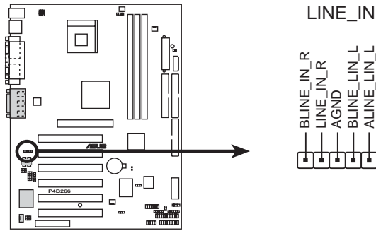
P4B266 LINE_IN Connector
