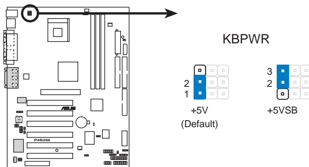
P4B266 Keyboard Power Setting
