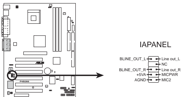
P4B266 Front Panel Audio Connector
