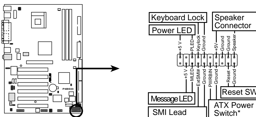
P4B533 System Panel Connectors * Requires an ATX power supply.
