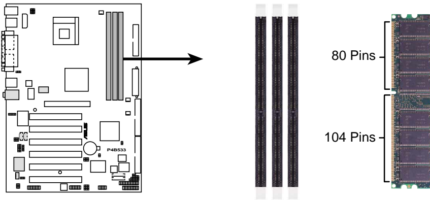
P4B533 184-Pin DDR DIMM Sockets
