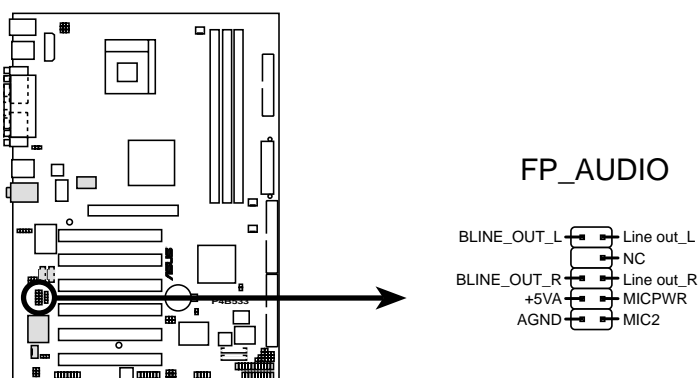
P4B533 Front Panel Audio Connector
