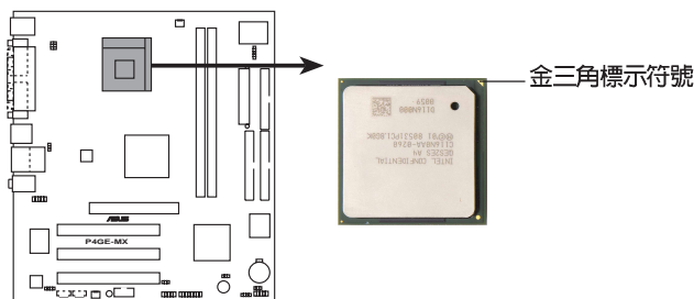
P4GE-MX CPU Socket 478
