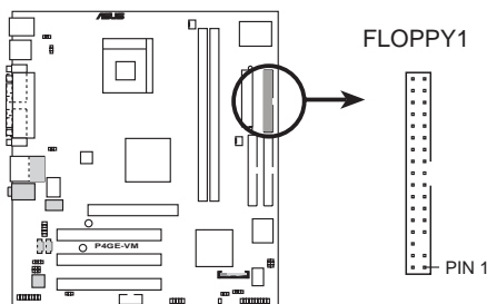
P4GE-VM Floppy Disk Drive Connector
