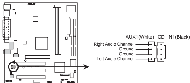
P4GE-VM Internal Audio Connectors
