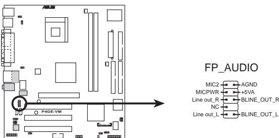
P4GE-VM Front Panel Audio Connector
