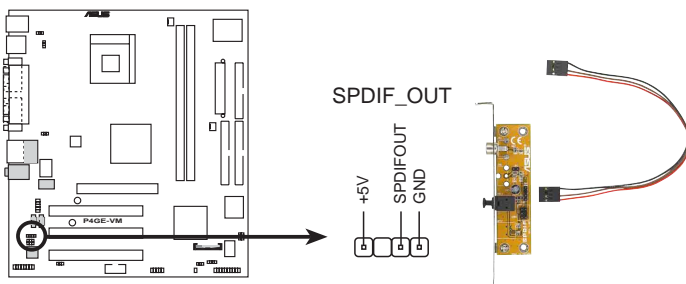
P4GE-VM Digital Audio Connector
