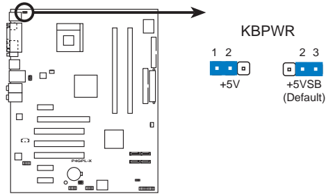
P4GPL-X Keyboard power setting
