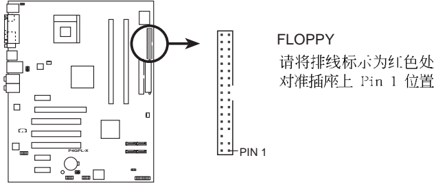
P4GPL-X Floppy disk drive connector
