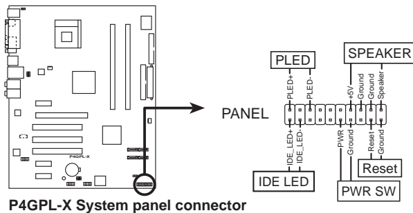
P4GPL-X System panel connector
