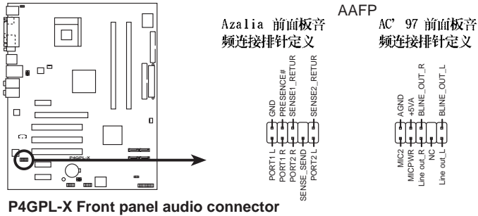
P4GPL-X Front panel audio connector
