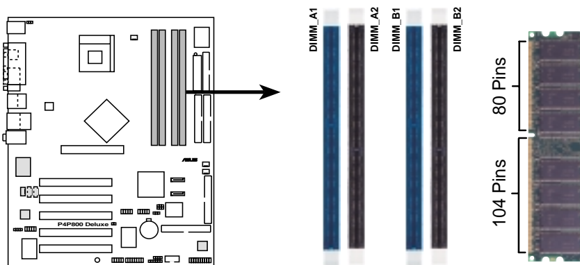
P4P800 184-Pin DDR DIMM Sockets
