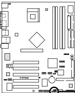
P4P800 SMBus Connector
