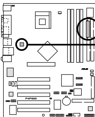
P4P800 ATX Power Connector
