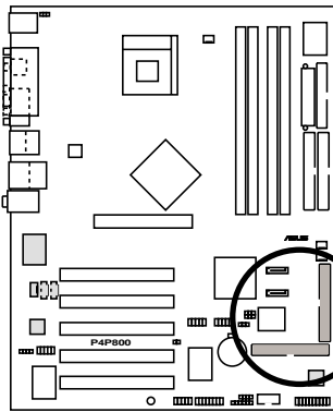
P4P800 RAID Connectors
