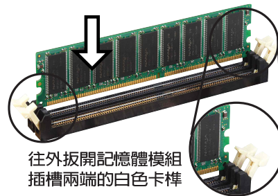
P4P800 184-Pin DDR DIMM Sockets
