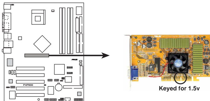
P4P800 Accelerated Graphics Port (AGP)
