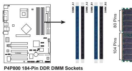
P4P800 184-Pin DDR DIMM Sockets
