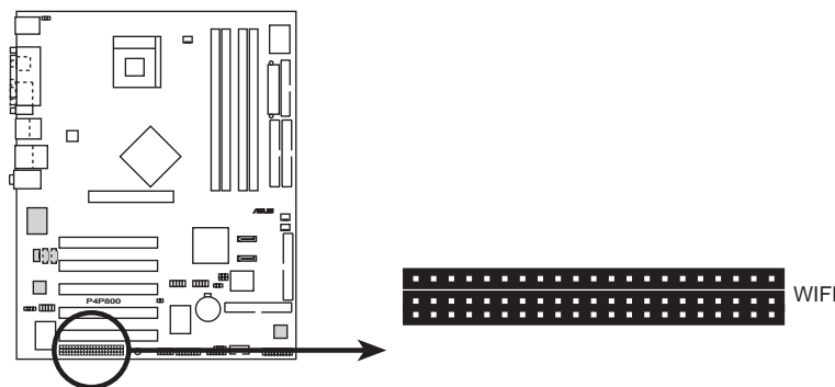
P4P800 WIRELESS Connectors
