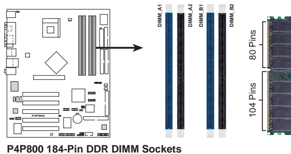
P4P800 184-Pin DDR DIMM Sockets
