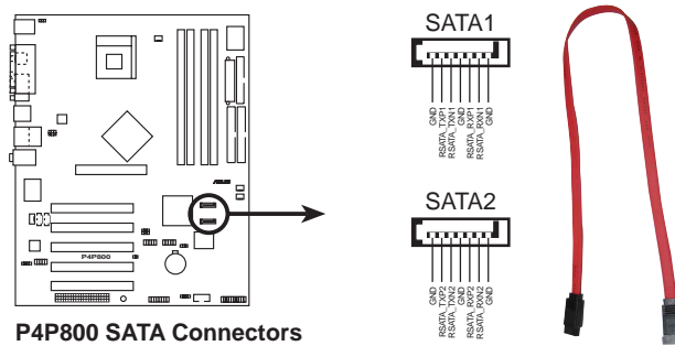
P4P800 SATA Connectors
