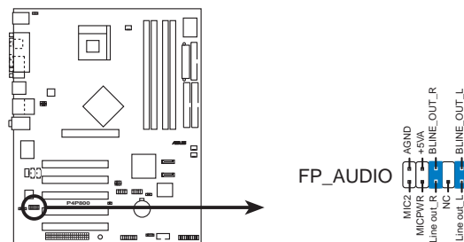
P4P800 Front Panel Audio Connector
