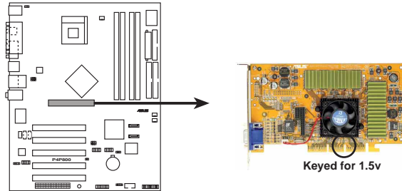
P4P800 Accelerated Graphics Port (AGP)
