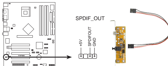
P4P800 Digital Audio Connector
