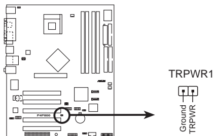
P4P800 Power Supply Thermal Connector
