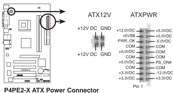
P4PE2-X ATX Power Connector
