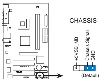
P4PE2-X Chassis Alarm Lead
