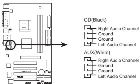
P4PE2-X Internal Audio Connectors
