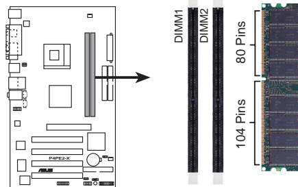
P4PE2-X 184-Pin DDR DIMM Sockets
