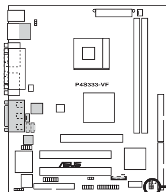
P4S333-VF IDE Activity LED
