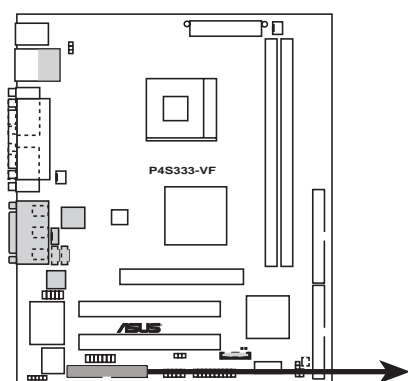
P4S333-VF Floppy Disk Drive Connector
