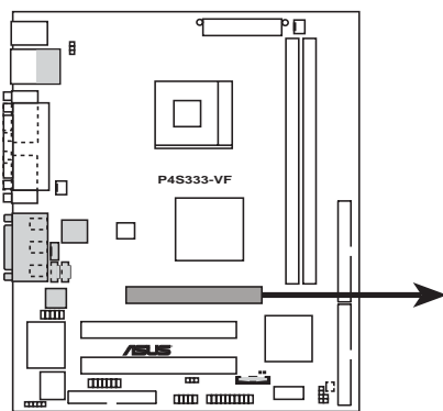
P4S333-VF Accelerated Graphics Port (AGP)
