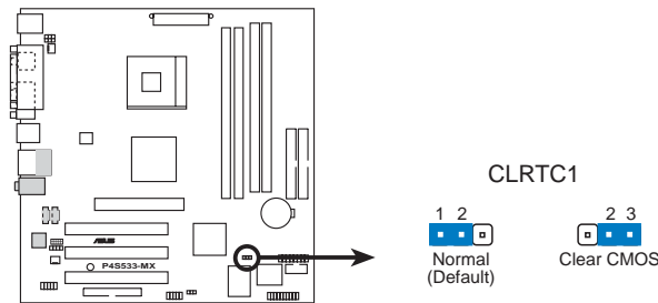
P4S533-MX Clear RTC RAM Setting
