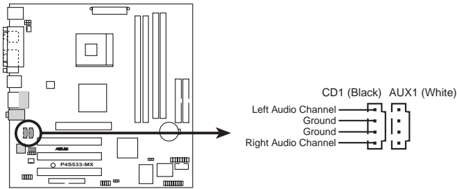
P4S533-MX Internal Audio Connectors
