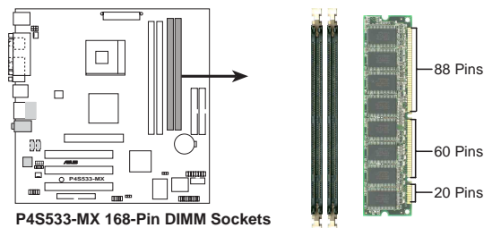
P4S533-MX 168-Pin DIMM Sockets
