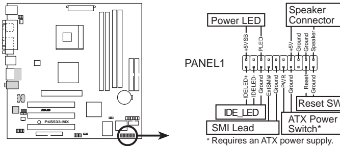
P4S533-MX System Panel Connectors
