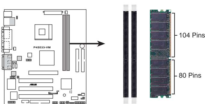
P4S533-VM 184-Pin DDR DIMM Sockets
