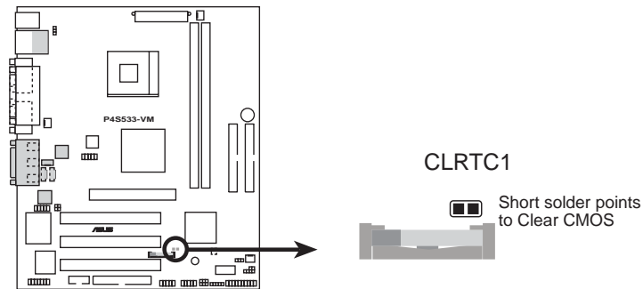
P4S533-VM Clear RTC RAM Setting
