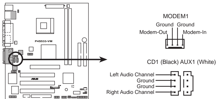
P4S533-VM Internal Audio Connectors
