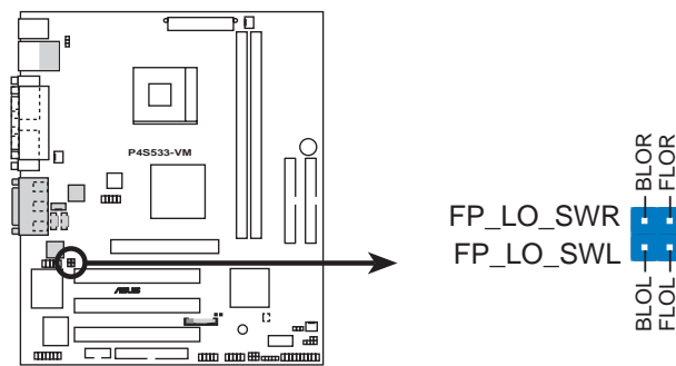
P4S533-VM Internal Line Out Connectors
