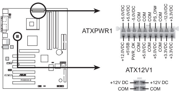
P4S533-X ATX Power Connectors
