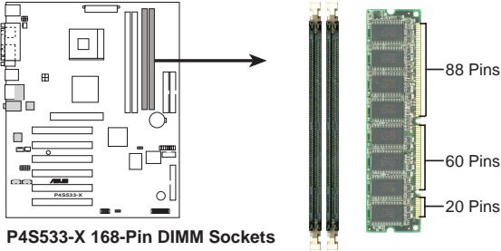
P4S533-X 168-Pin DIMM Sockets
