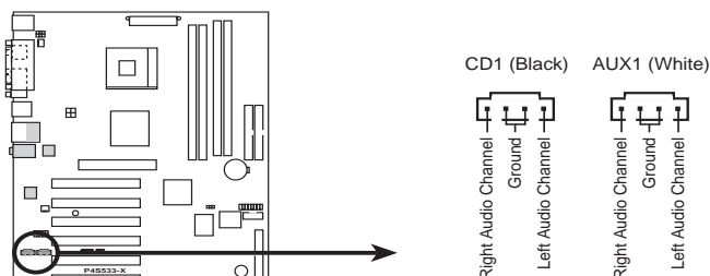
P4S533-X Internal Audio Connectors
