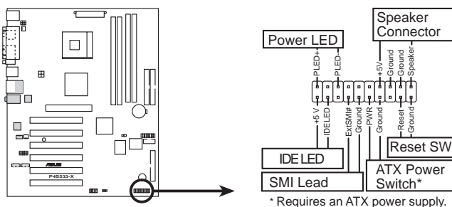
P4S533-X System Panel Connectors
