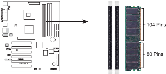
P4S533-X 184-Pin DDR DIMM Sockets
