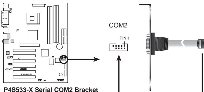
P4S533-X Serial COM2 Bracket
