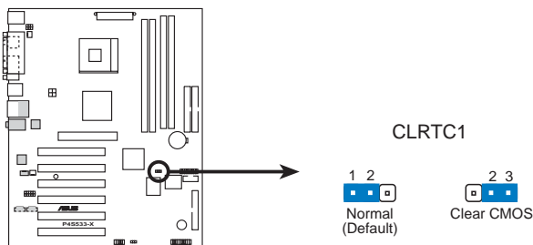
P4S533-X Clear RTC RAM Setting
