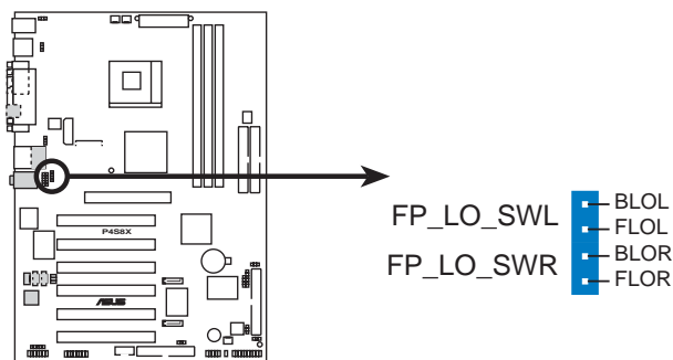
P4S8X Internal Line Out Selector
