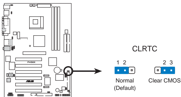
P4S8X Clear RTC RAM
