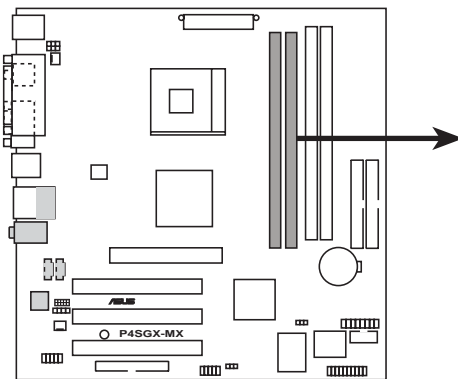
P4SGX-MX 184-Pin DDR DIMM Sockets
