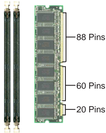
P4SGX-MX 168-Pin DIMM Sockets
