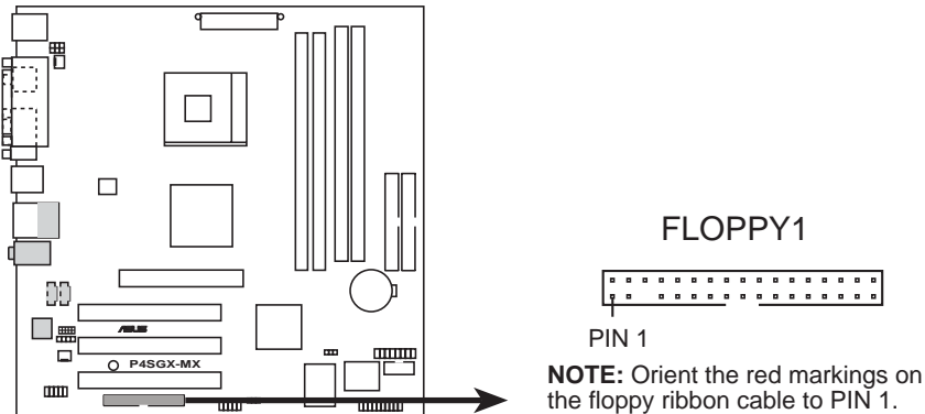
P4SGX-MX Floppy Disk Drive Connector
