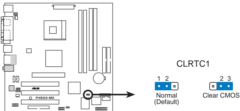
P4SGX-MX Clear RTC RAM Setting
