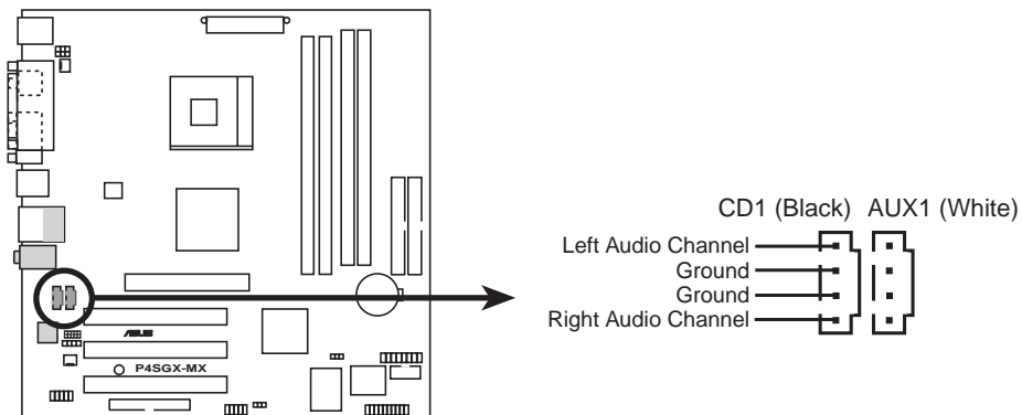
P4SGX-MX Internal Audio Connectors
